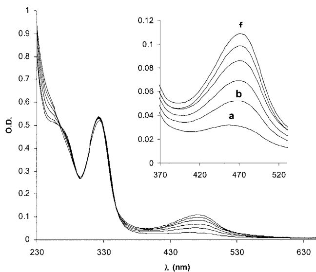
Figure 3. UV-visible titration of [(\text{CuCl}_2)_2 \cdot \mathbf{6}] by ascorbic acid: a) [(\text{CuCl}_2)_2 \cdot \mathbf{6}] , [2 mL; 2.0 \times 10^{-5} M in \text{H}_2\text{O} ]; from b) to f): addition of 0.5 equiv. of ascorbic acid [ 5 \times 4 \mu\text{L} ; 1.00 \times 10^{-3} M in \text{H}_2\text{O} ]
