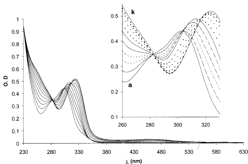
Figure 2. UV-visible titration of 6 by \text{CuCl}_2 \cdot 2\text{H}_2\text{O} : a) 6 , [2 mL; 2.0 \times 10^{-5} M in \text{H}_2\text{O} ]; from b) to k): addition of 2 equiv. of \text{CuCl}_2 \cdot 2\text{H}_2\text{O} [ 10 \times 8 \mu\text{L} ; 1.00 \times 10^{-3} M in \text{H}_2\text{O} ]
