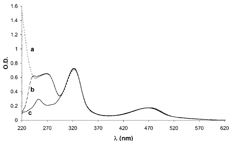
Figure 4. UV-visible analysis of 7 in the presence of bovine serum albumin: a) 7 , [ 1.6 \times 10^{-5} M in \text{H}_2\text{O} ]; b) 1 equiv. of BSA; c) 10 equiv. of BSA
