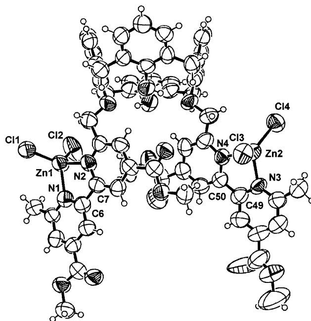
Figure 7. ORTEP side-view of complex 9 , molecule C
