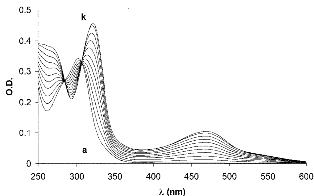
Figure 1. UV-visible titration of 6 with [Cu(MeCN) 4 ]PF 6 : a) 6 , [2 mL; 1.71 × 10 -5 M in H 2 O]; from b) to k): addition of 1 equiv. of [Cu(MeCN) 4 ]PF 6 [10 × 4 μL; 9.98 × 10 -4 M in MeCN]
