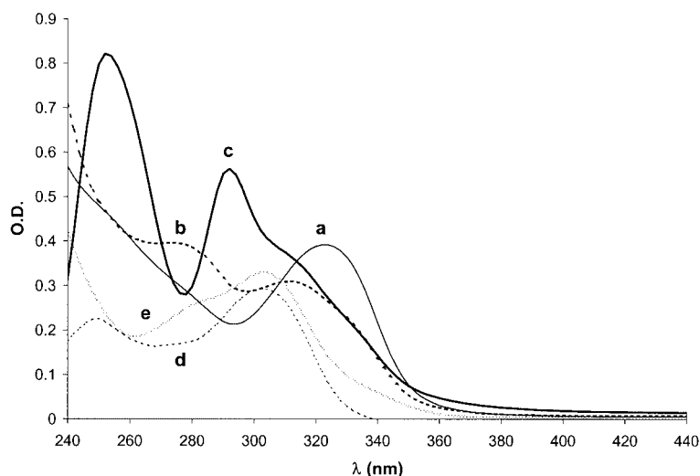
Figure 5. UV-visible analysis of [(\text{CuCl}_2)_2 \cdot \mathbf{6}] in the presence of bovine serum albumin: a) [(\text{CuCl}_2)_2 \cdot \mathbf{6}] , [ 1.6 \times 10^{-5} M in \text{H}_2\text{O} ]; b) 1 equiv. of BSA; c) 10 equiv. of BSA; d) 10 equiv. of BSA, one day; e) 6 [ 1.6 \times 10^{-5} M in \text{H}_2\text{O} ]
