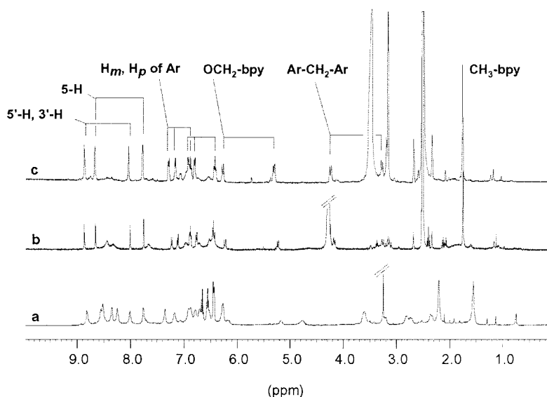
Figure 6. ^1\text{H} NMR spectrum of the copper(I) complex 7 (a: \text{D}_2\text{O} , b: \text{D}_2\text{O} + [\text{D}_6]\text{DMSO} , c: [\text{D}_6]\text{DMSO} ; 400 MHz, room temp.)
